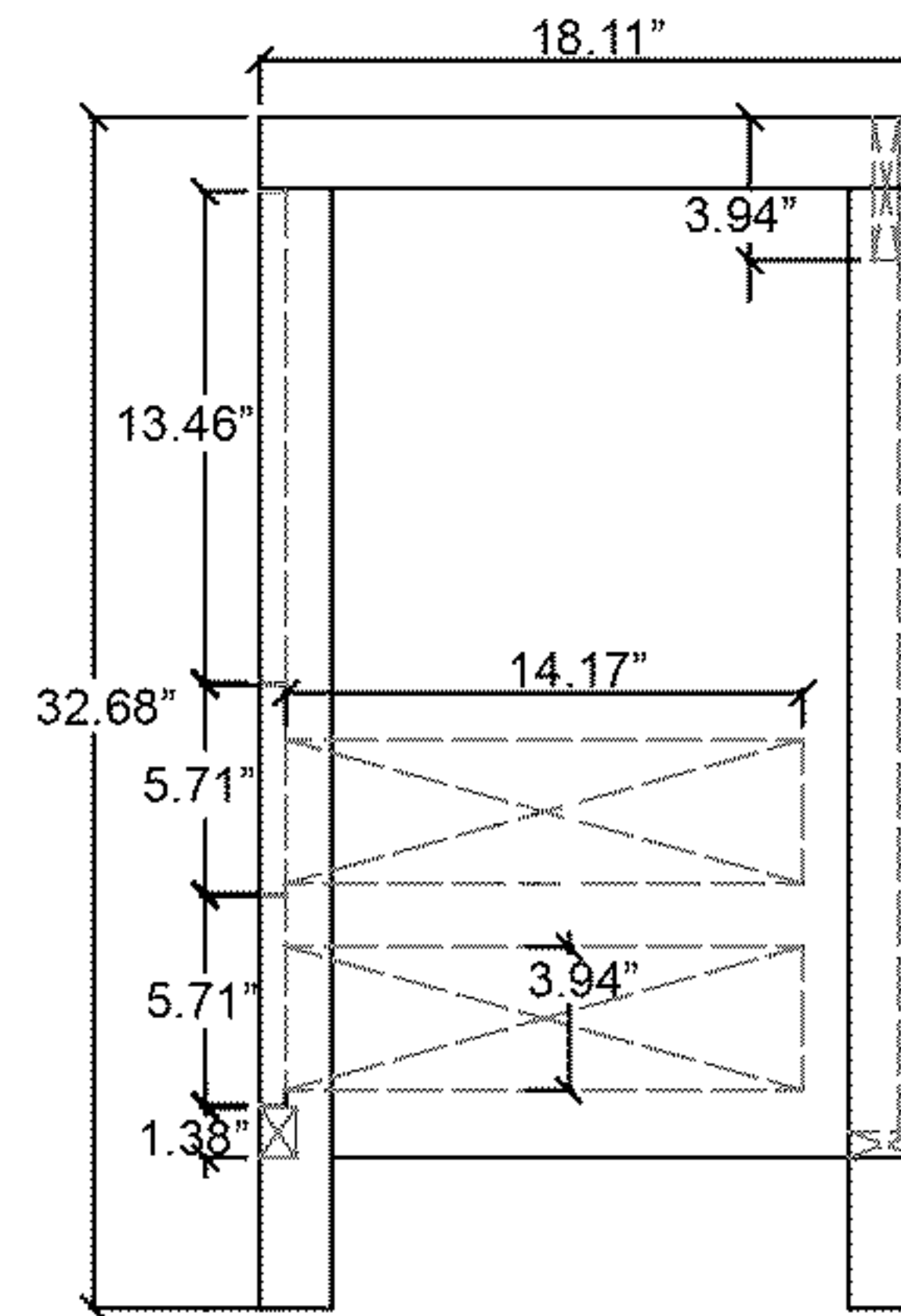
Side View
