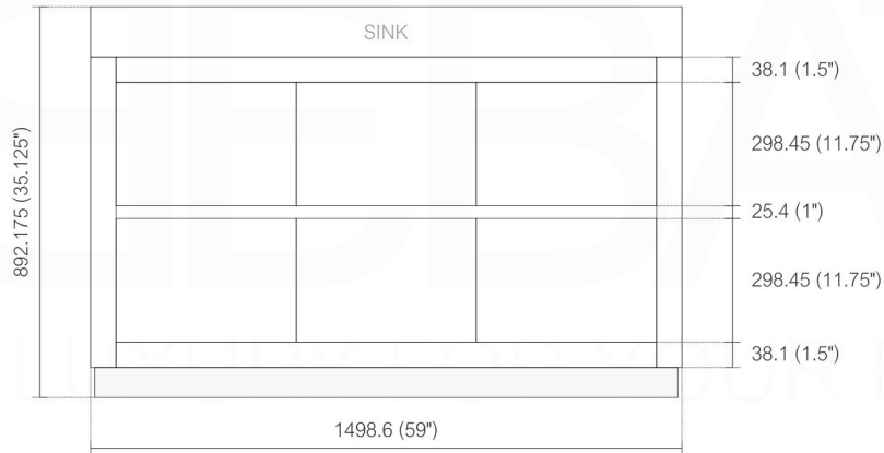
BACK ELEVATION
