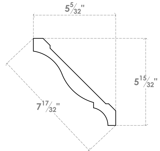
SIDE PROFILE
