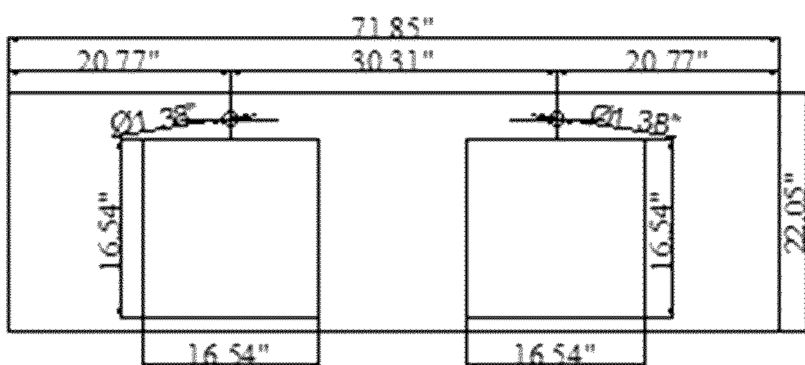
TOP VIEW
