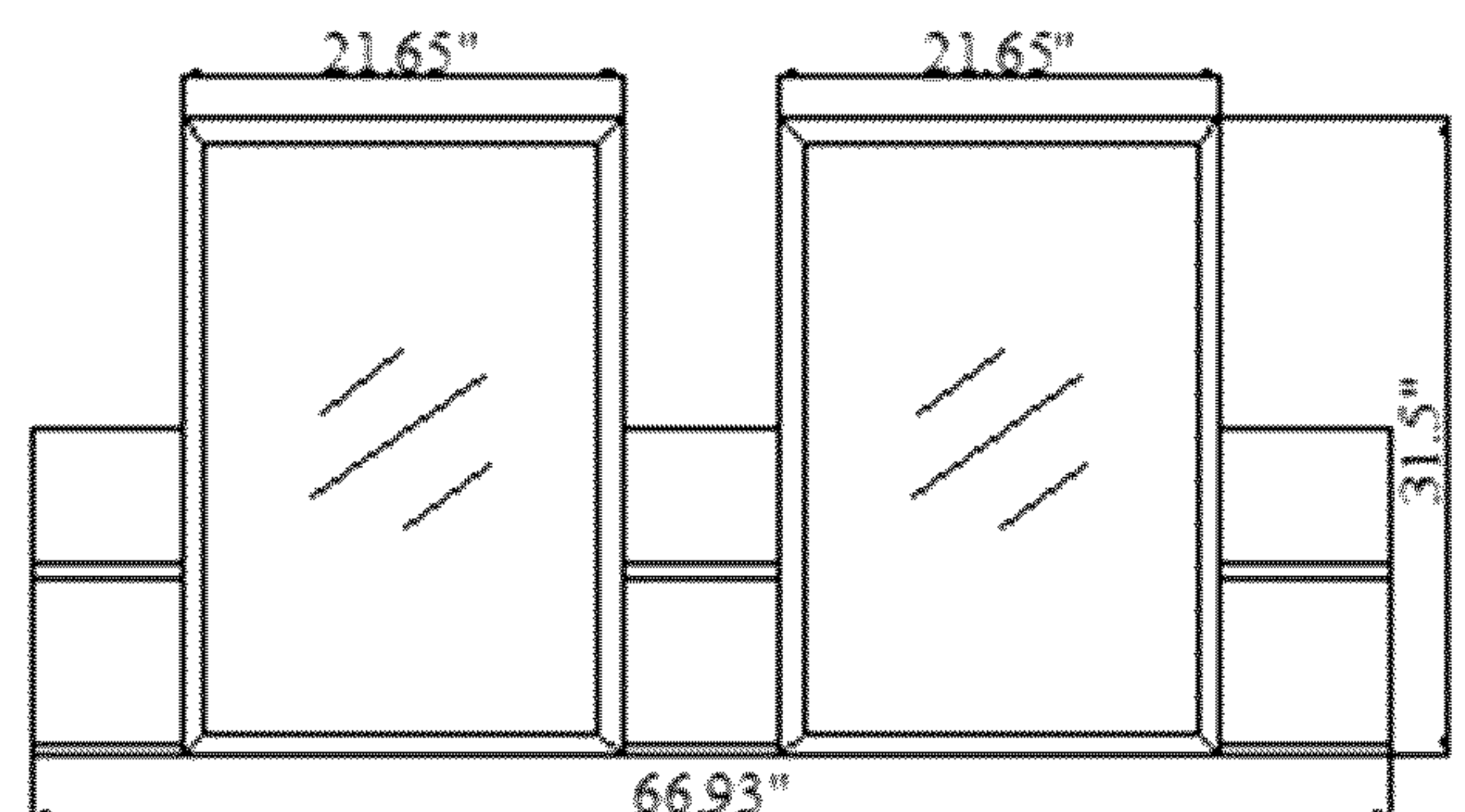
MIRROR VIEW
