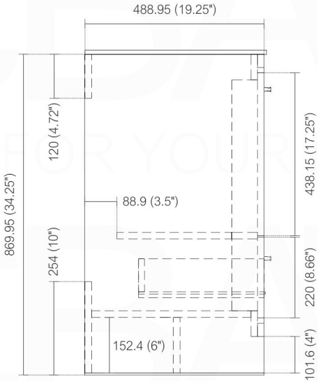
. SIDE ELEVATION
