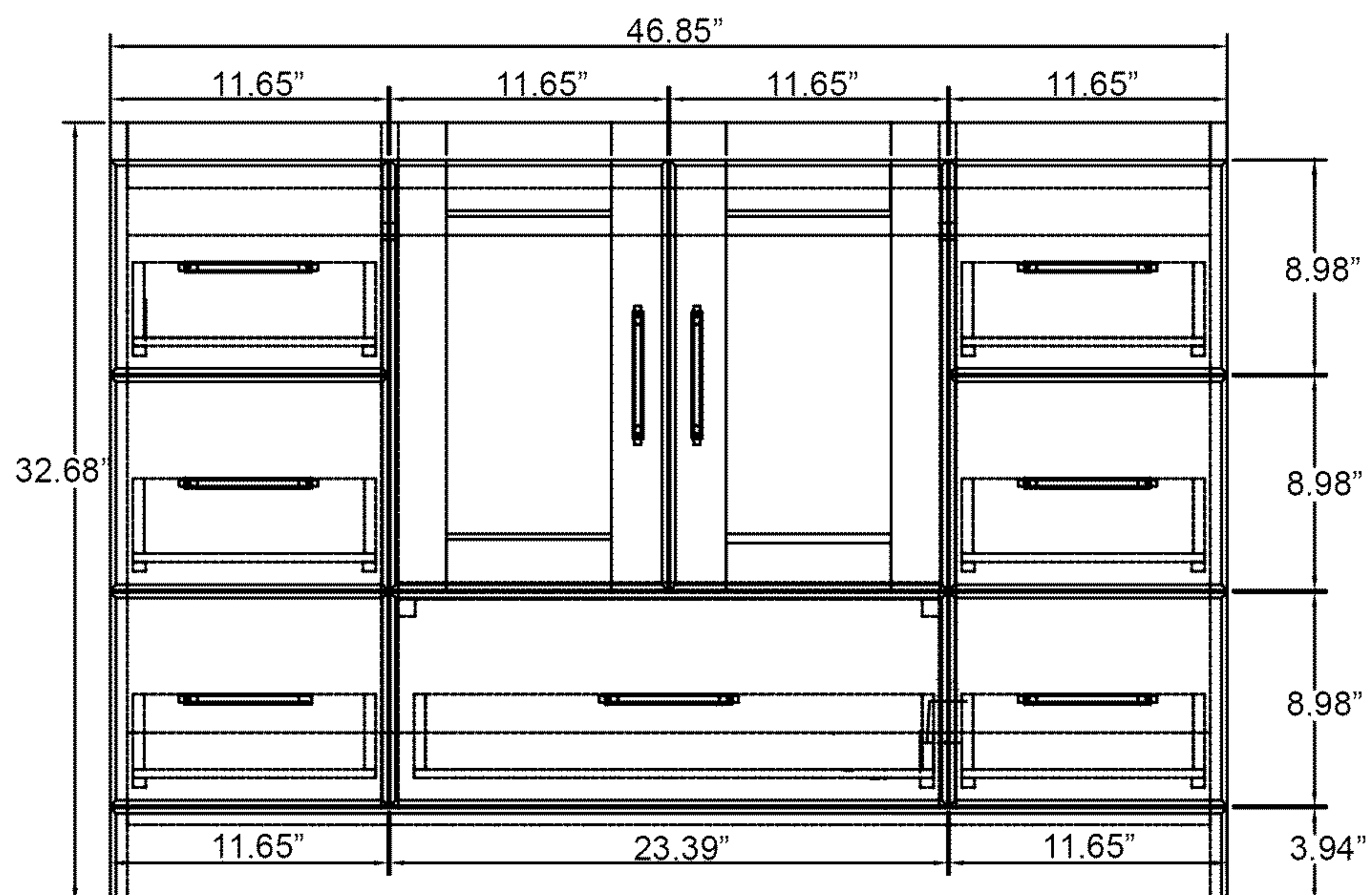
Front View
