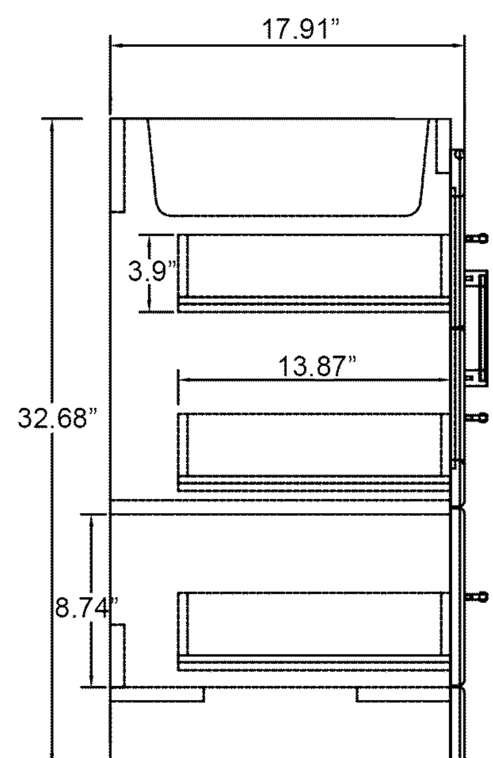
Side View
