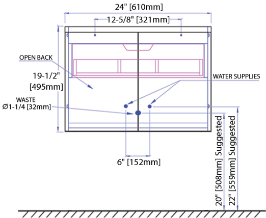
24" VANITY BACK VIEW (V8000 24)
