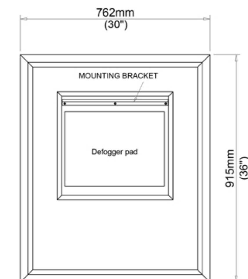
Back view for electrical knockout location
