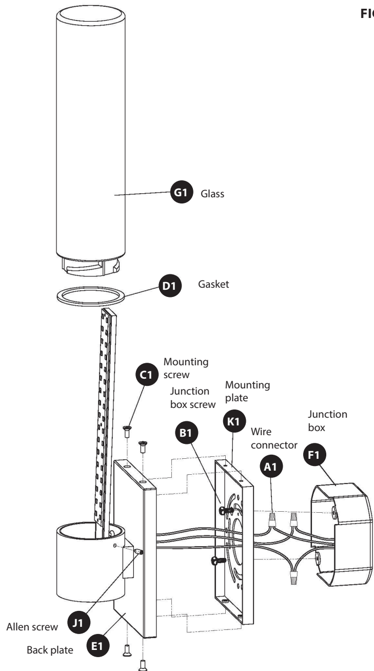
Fig.2 Wiring
