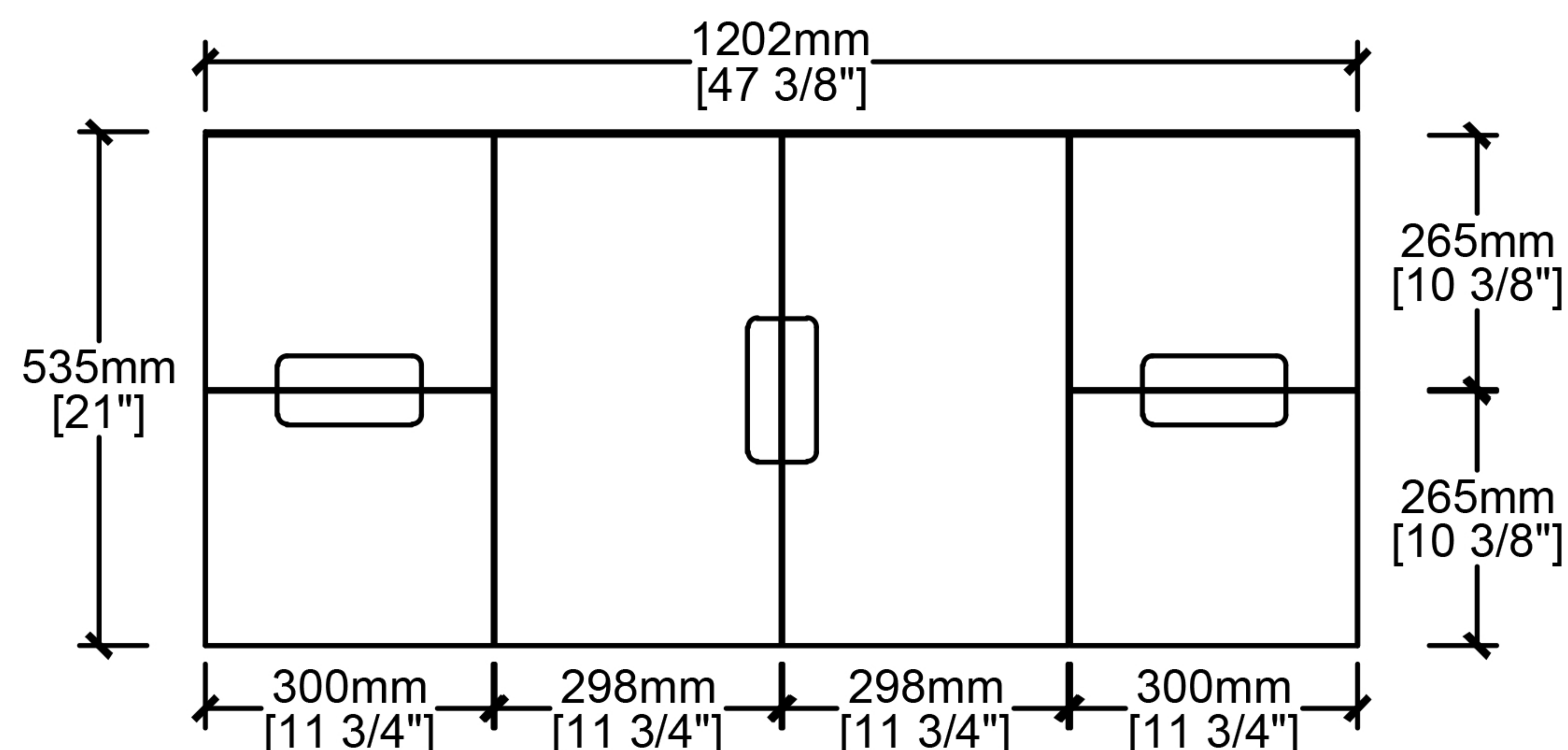
Front View
