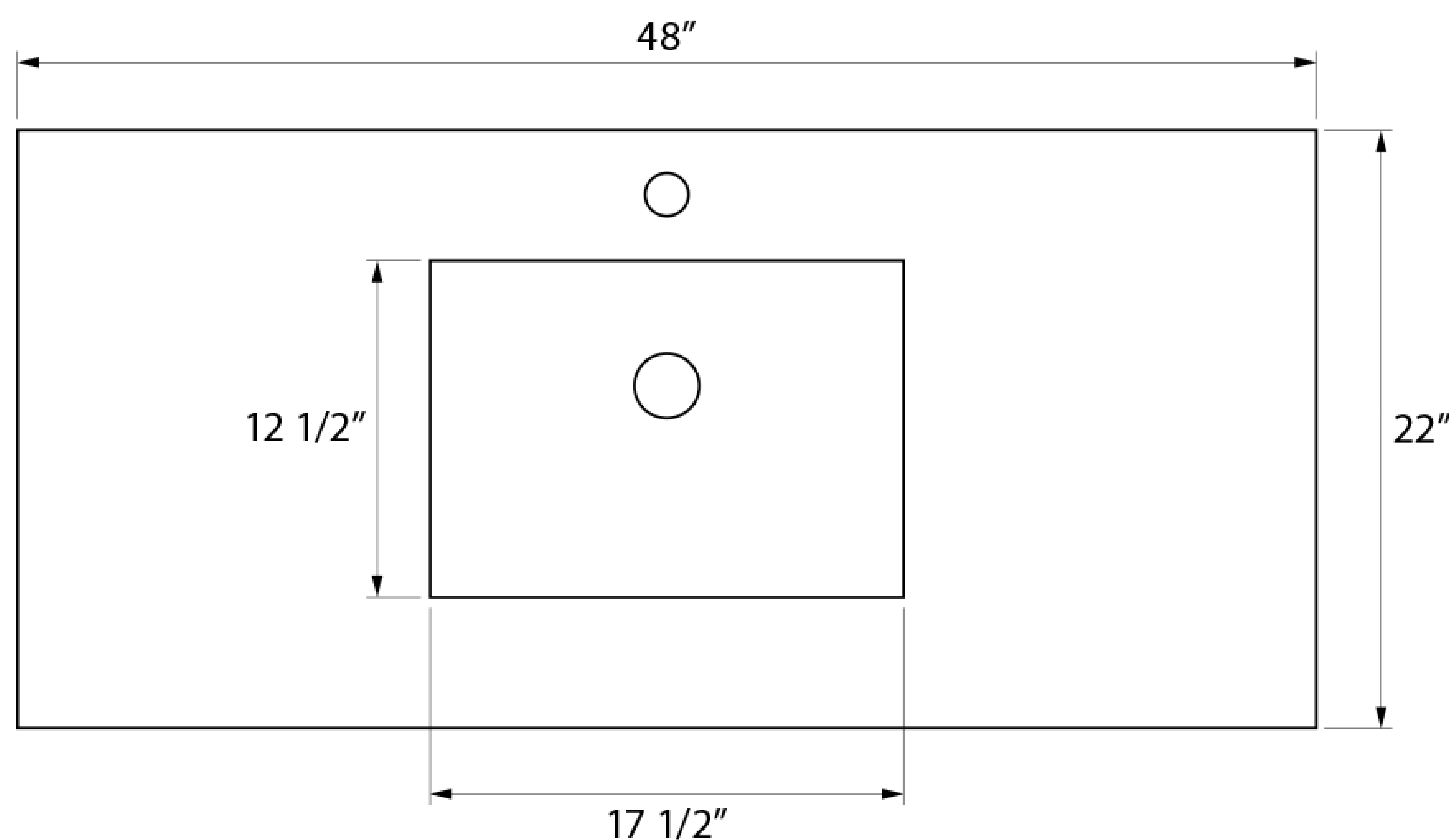
Top View
