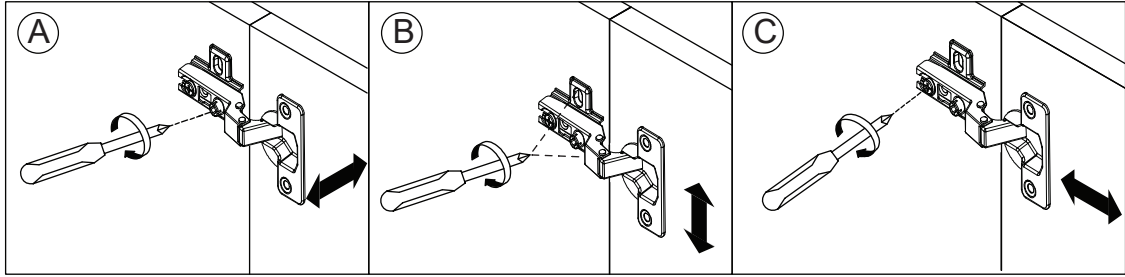
A. Lateral adjustment by screw adjusting B. Vertical adjustment via slot in the mounting plate C. Front-to-Back by slacking the hinge arm mounting screw
