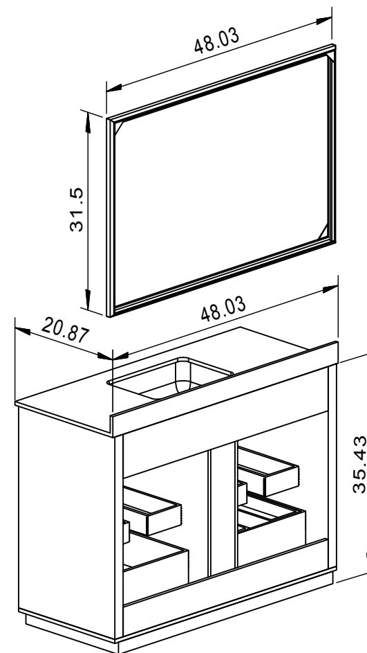
Back View
