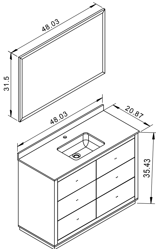
Isometric View
