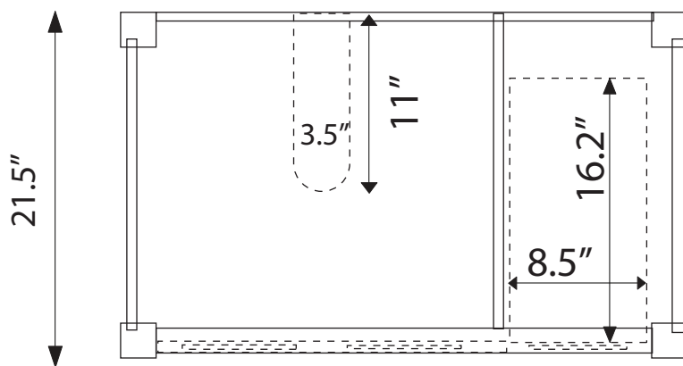
Top view (without countertop)
