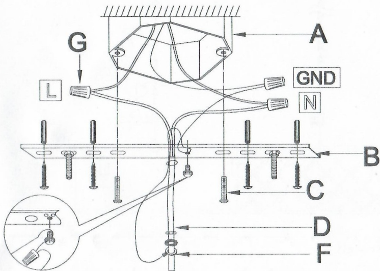
Wire Connection Diagram:
