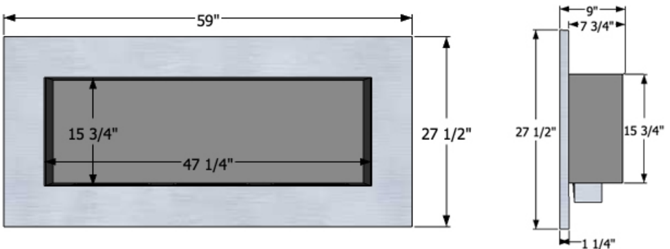
Optimum Fireplace Dimensions
