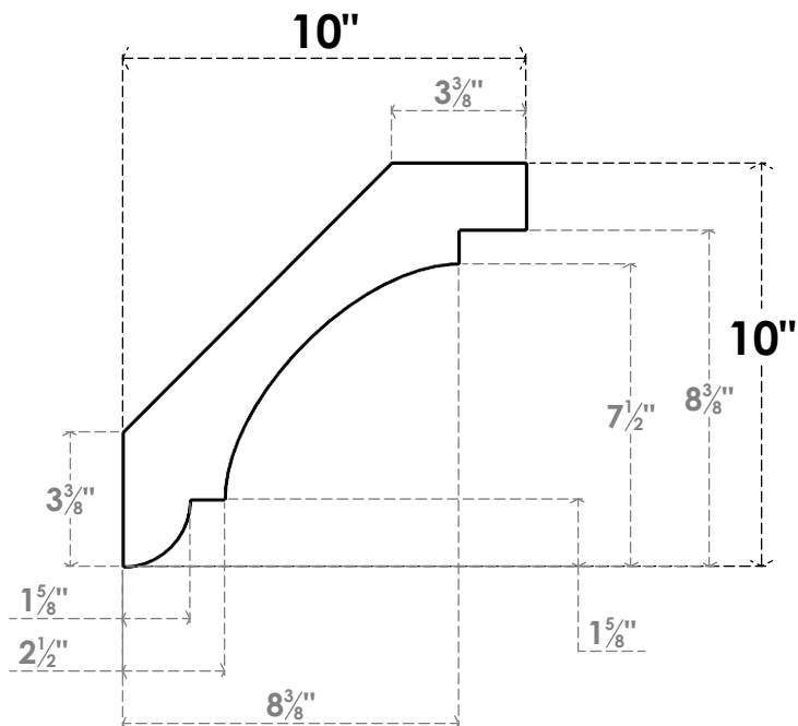
SIDE PROFILE
