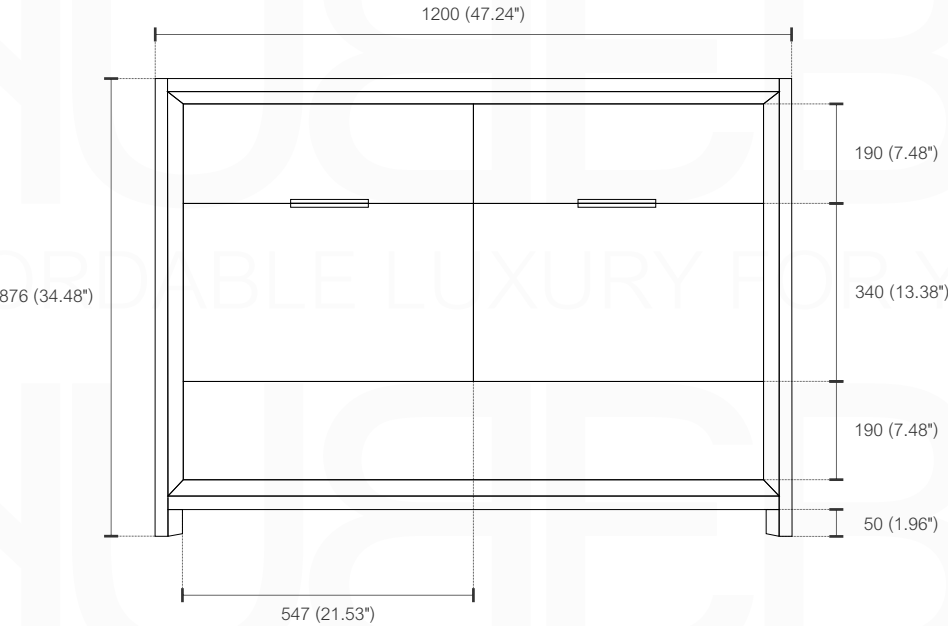
. FRONT ELEVATION
