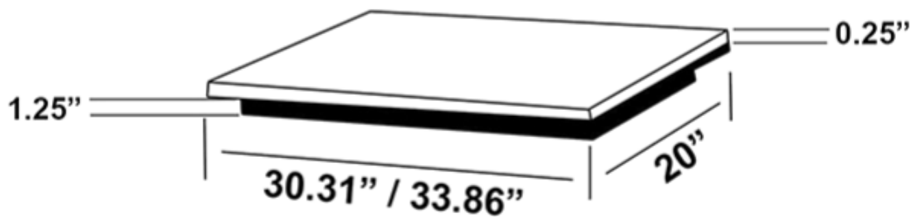
CUT-OUT VIEW
