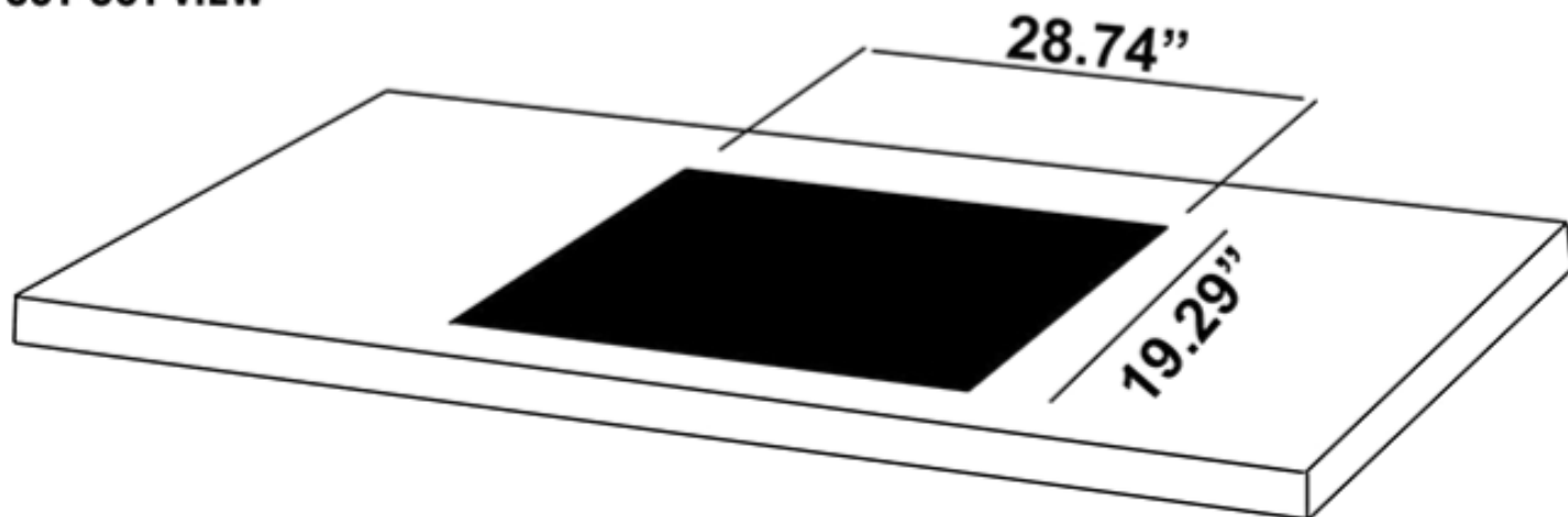
CUT-OUT VIEW
