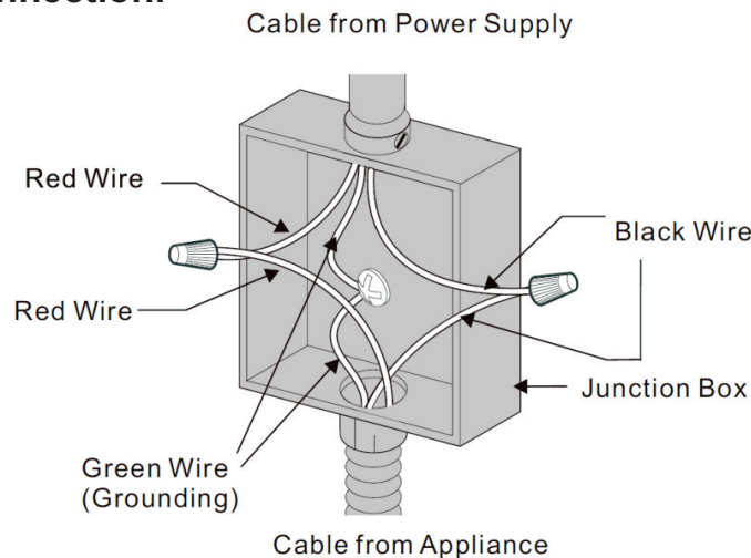
3-Wire Cable from Home Power Supply
