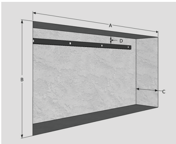
Recessed Opening Sized for Bellezza Fireplace
