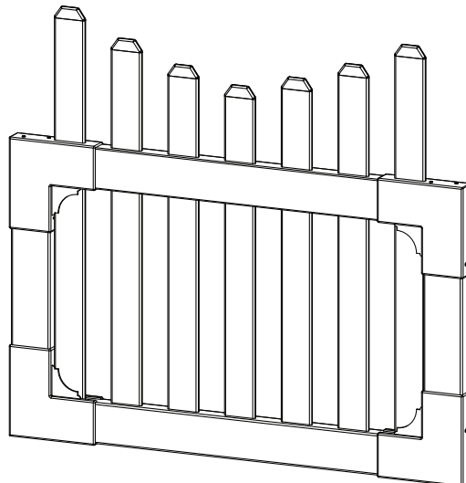
Assembled Gate
