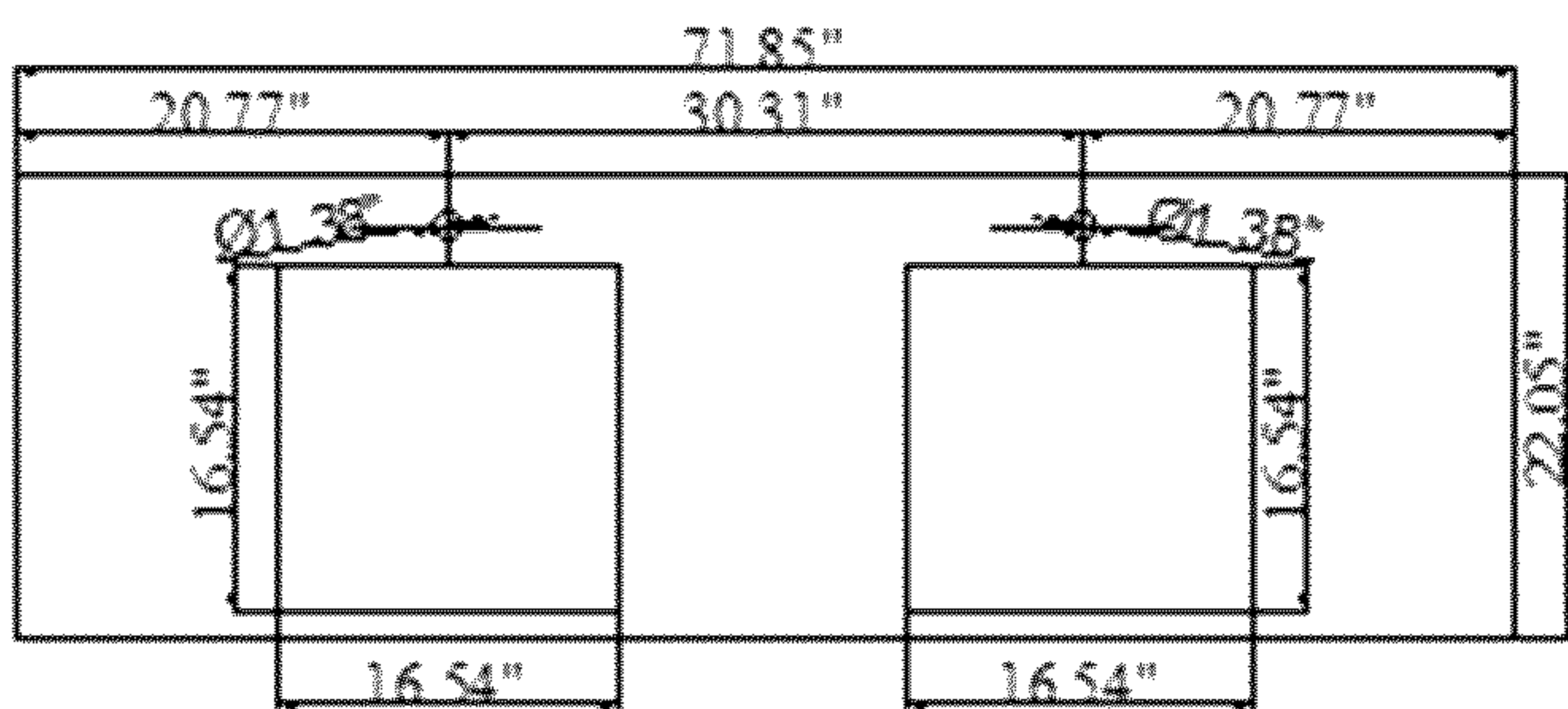
TOP VIEW
