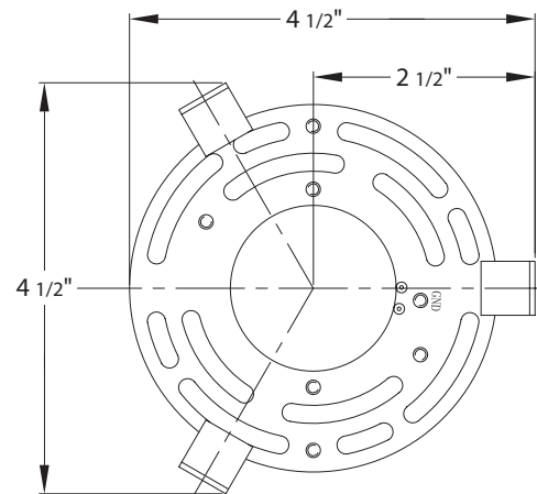
Back Plate Dimensions
