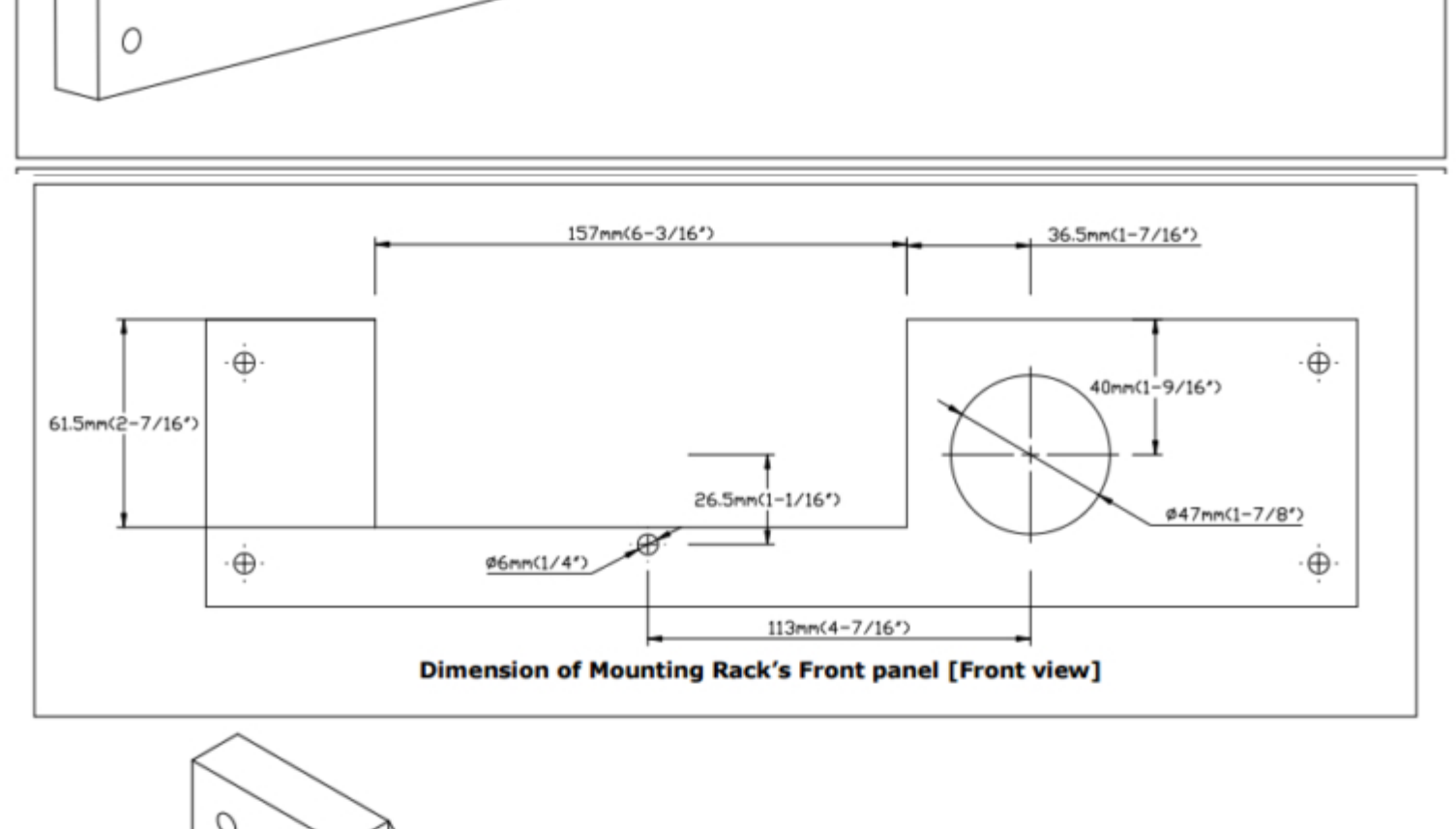
Dimension of Mounting Rack's Front panel [Front view]
