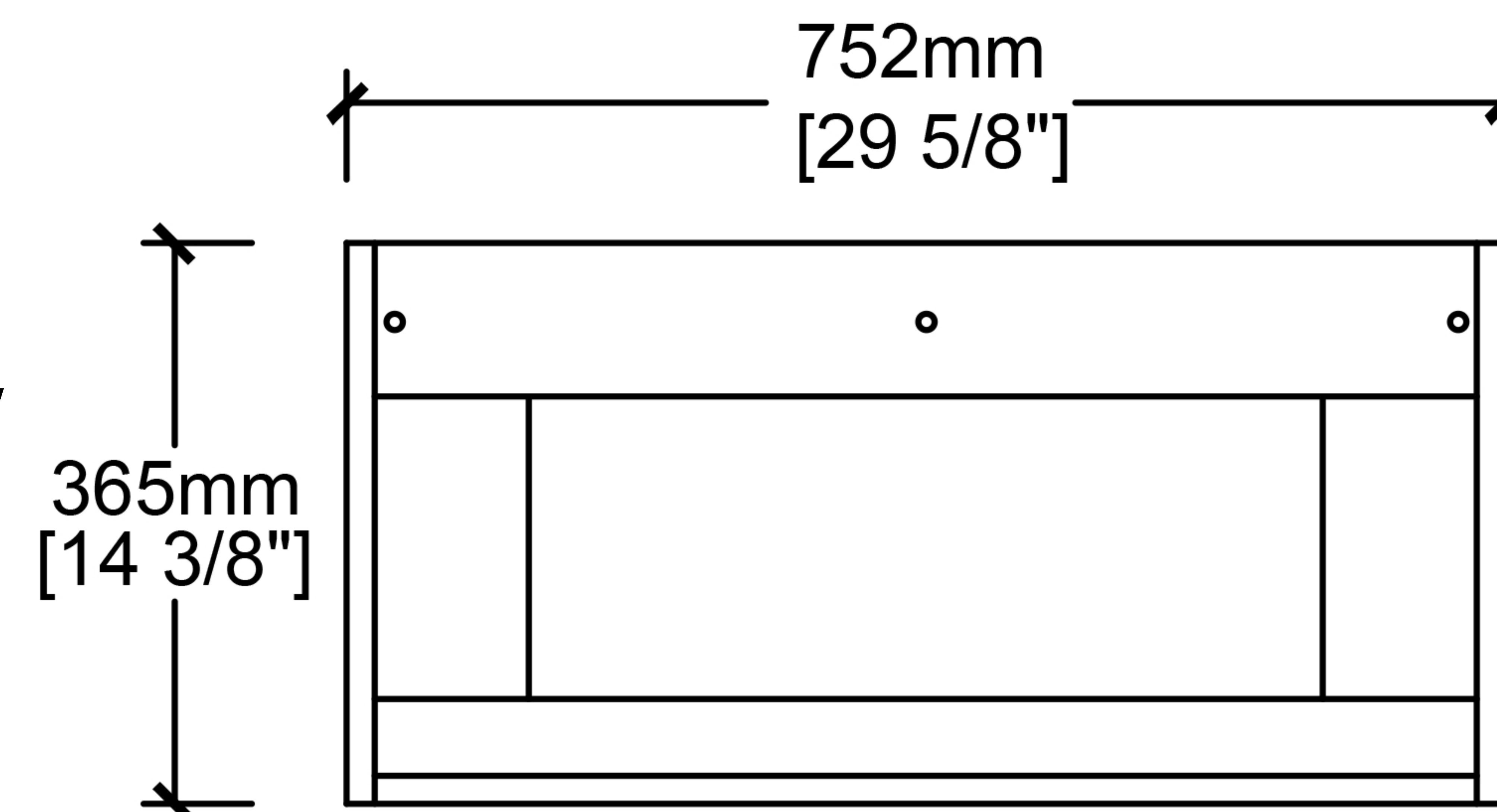
Rear View
