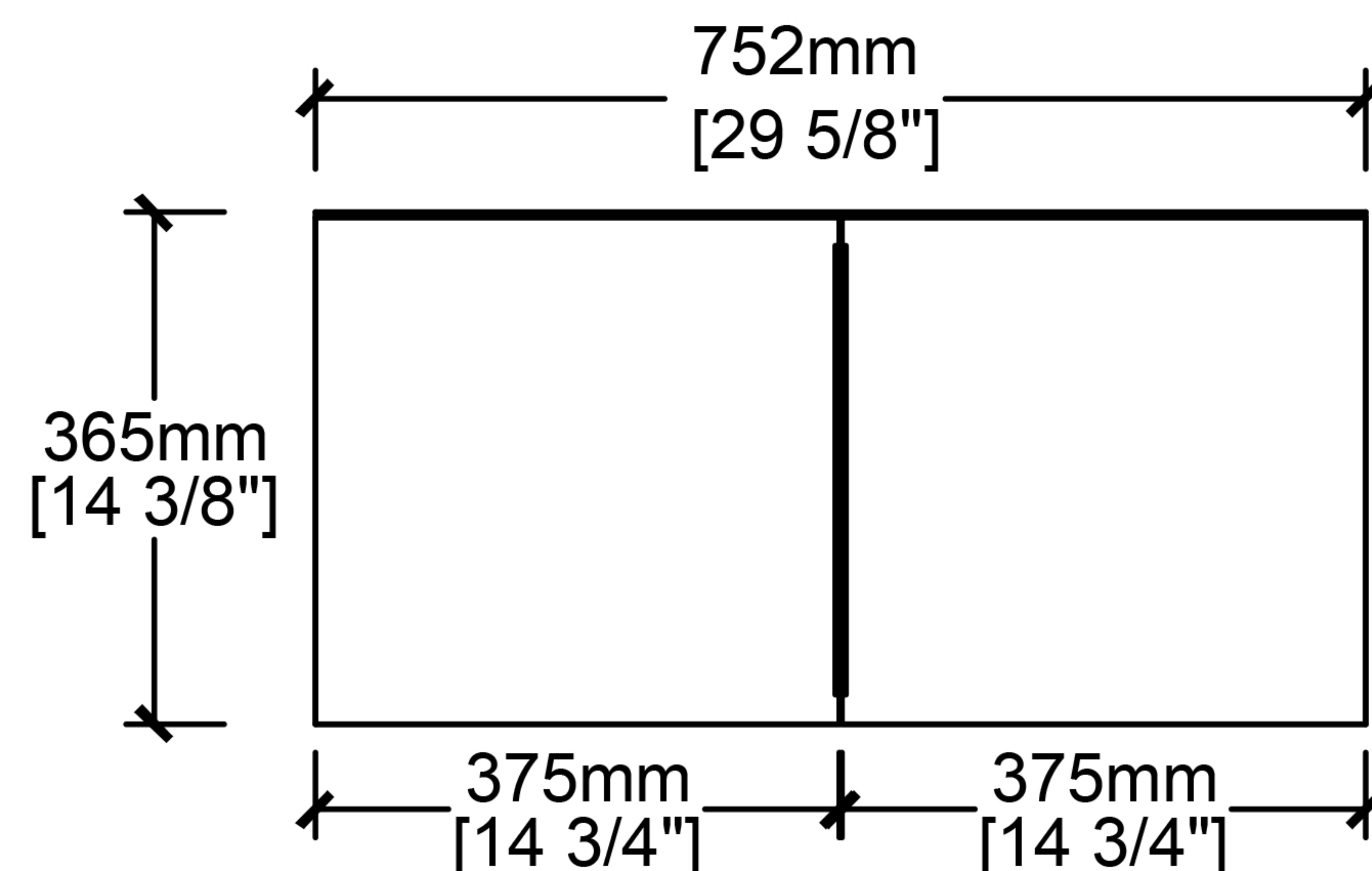
Front View
