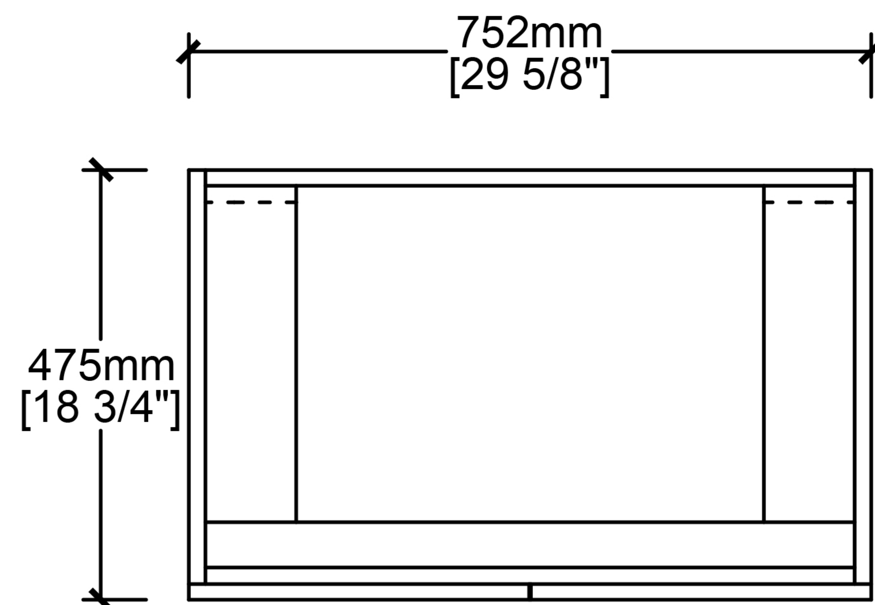
Top View
