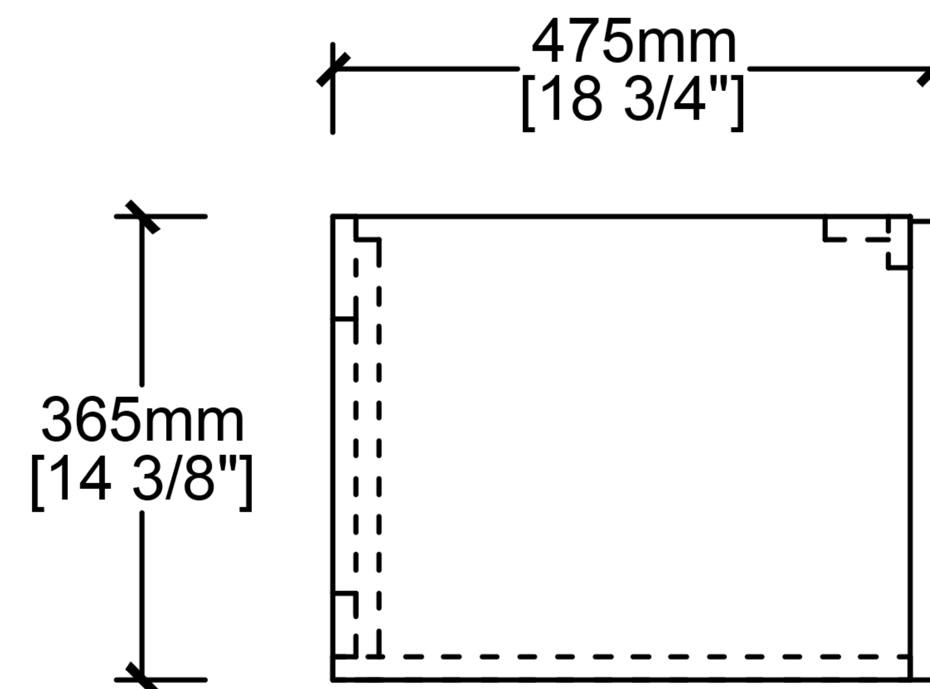
Side View
