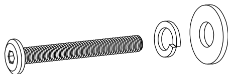
ALLEN KEY BOLT: M6 X 70mm - QTY 8 LOCK WASHER: Ø10 / Ø6 X 1.5mm - QTY 8 WASHER: Ø16 / Ø6 X 1mm - QTY 8 QTY 8 SETS
