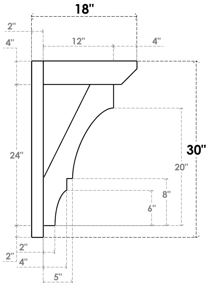
SIDE PROFILE
