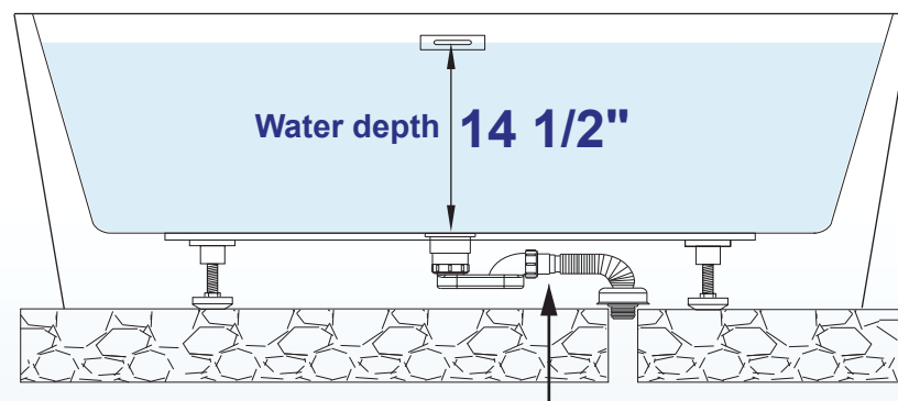
Anti-leak drain and pipe
