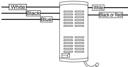
REMOTE CONTROL(1PCS)
