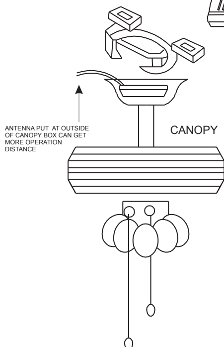
RECEIVER (FIG.4)
