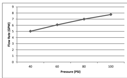
P-2302B Flow Rate (GPM) Vs Pressure (PSI) For Tub Port*
