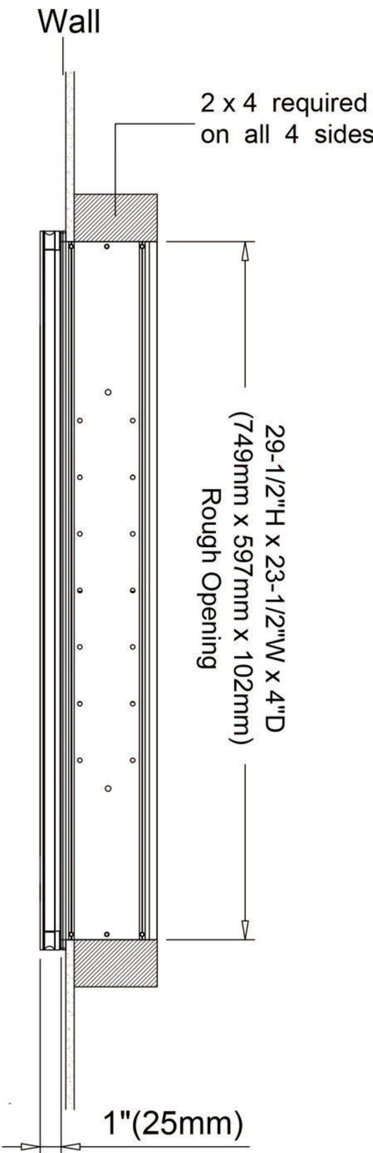
Recessed Mount
