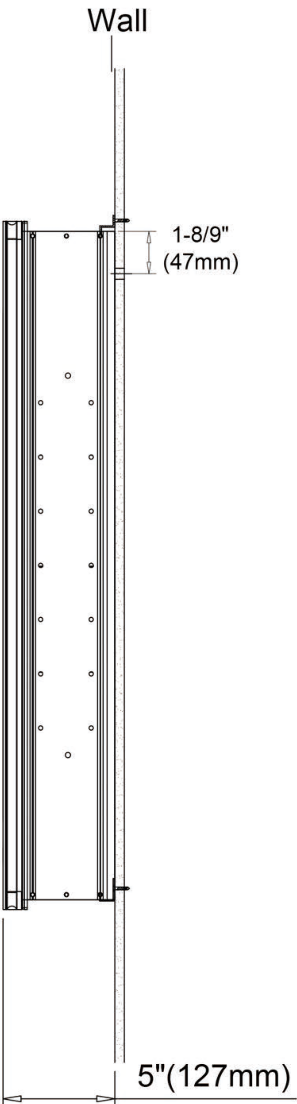
Surface Mount
