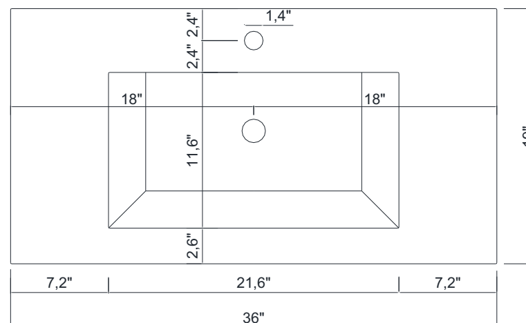
TOP WIEV
