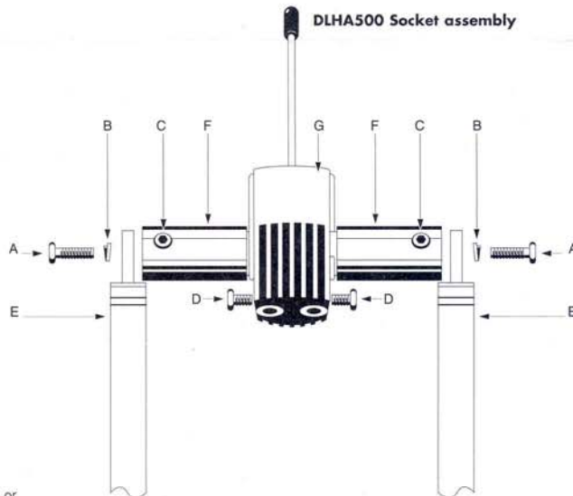
DLHA500 Socket assembly
