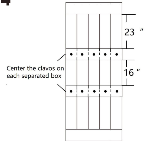
Assembled Door
