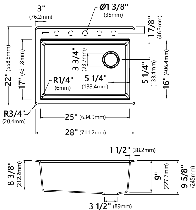
Model #: KGTW12-28 Sink Dimensions: 28" x 22" x 9 5/8" Min Cabinet Size: 30"
