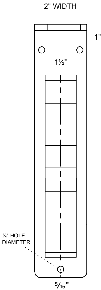
FRONT PROFILE
