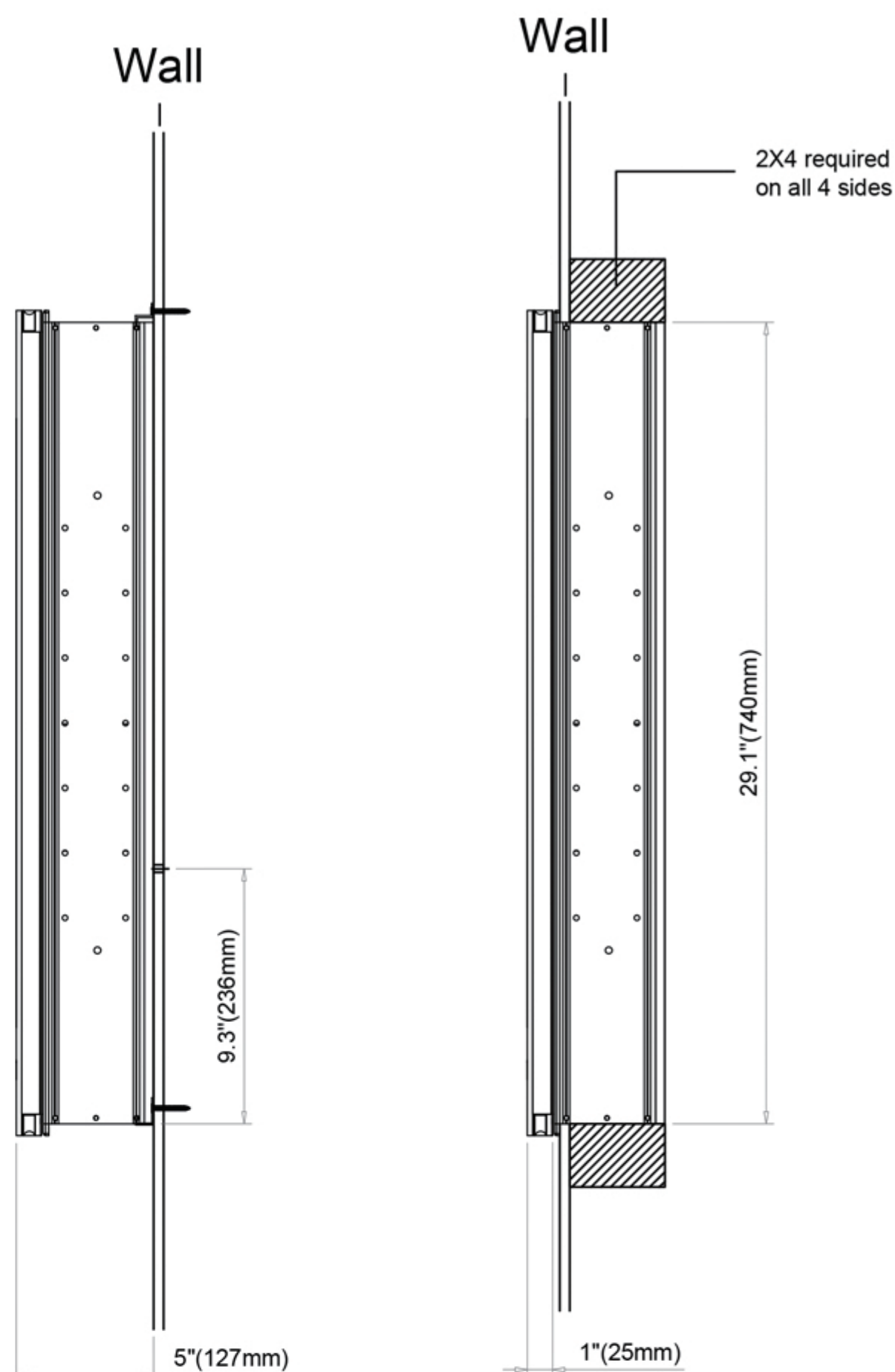
Surface Mount
