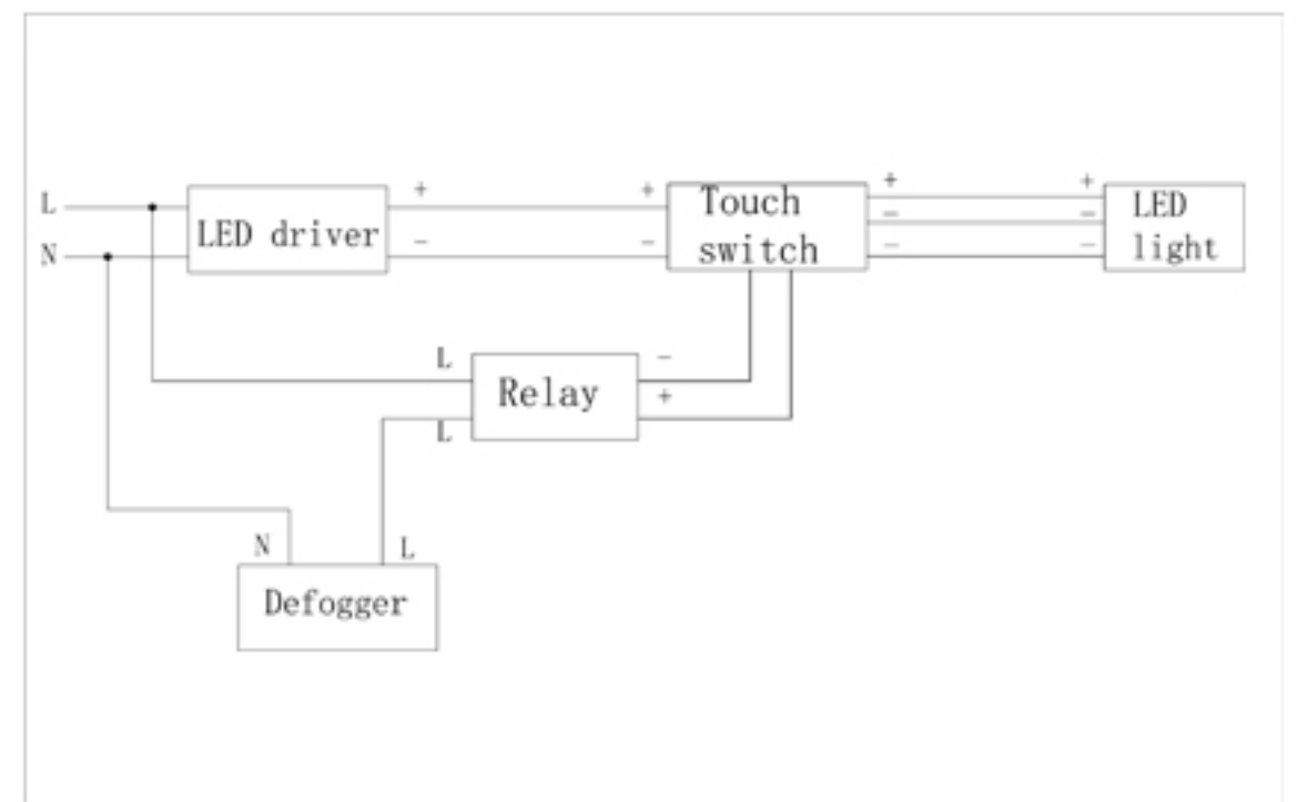
Circuit diagram
