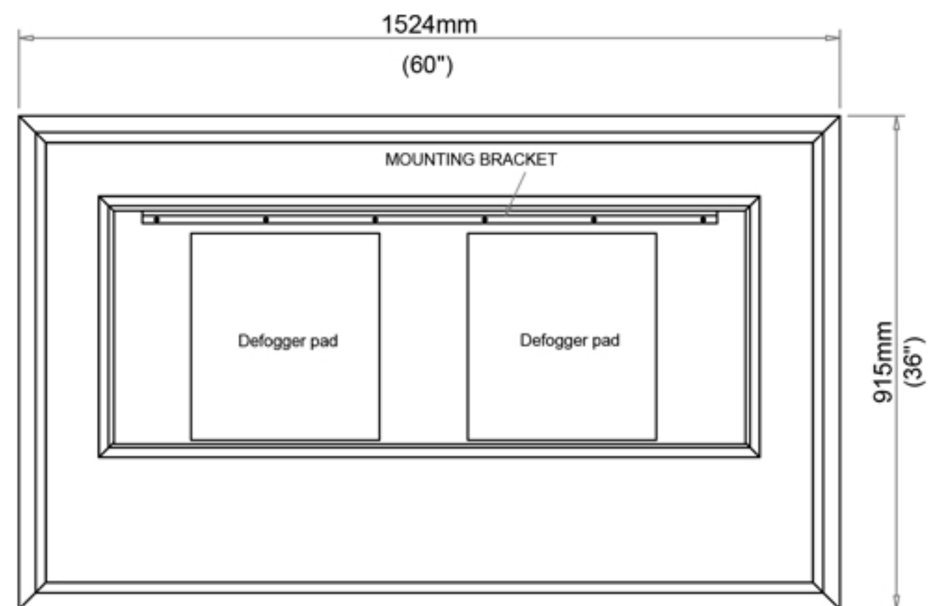
Back view for electrical knockout location
