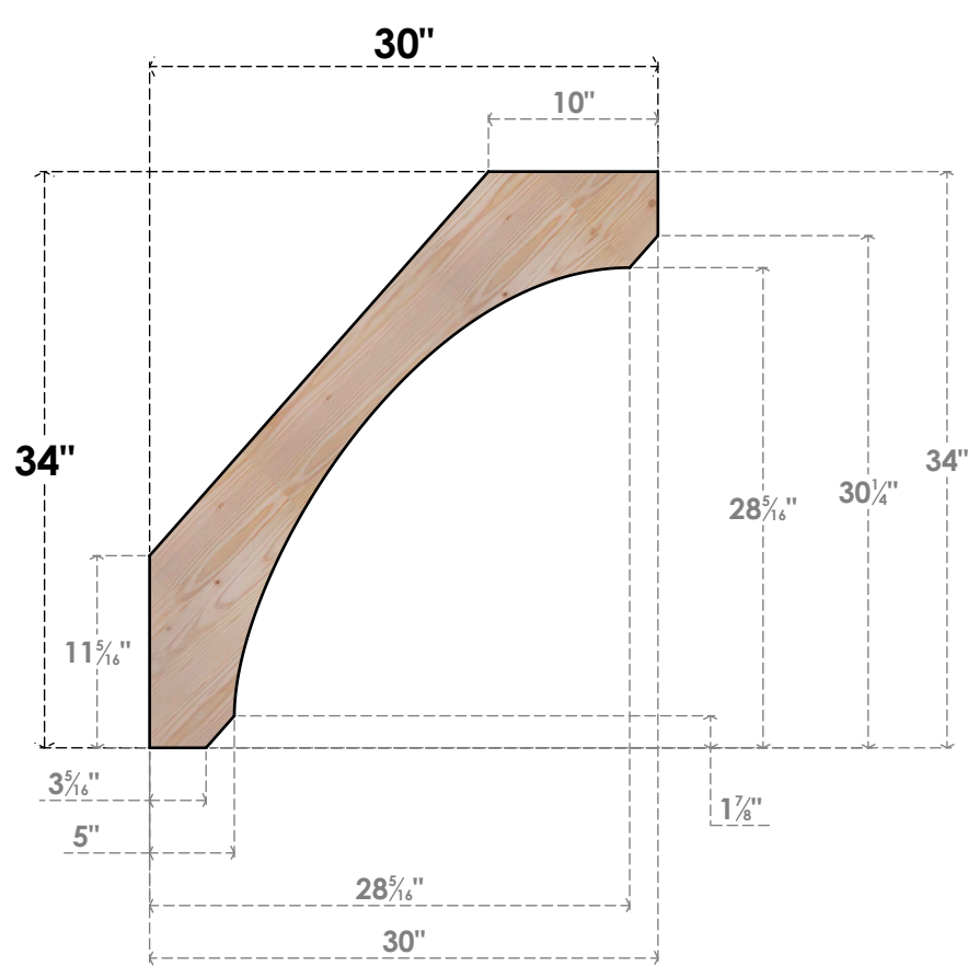
SIDE
