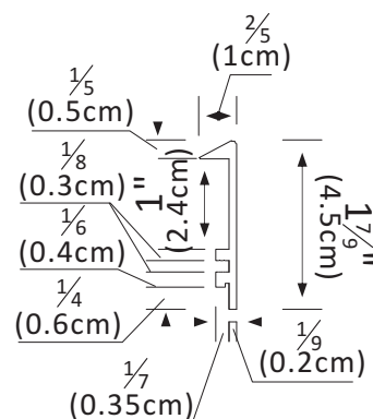
Aluminum section
