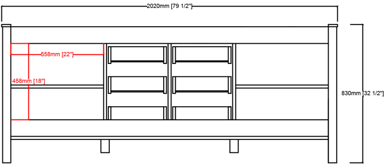
BACK VIEW
