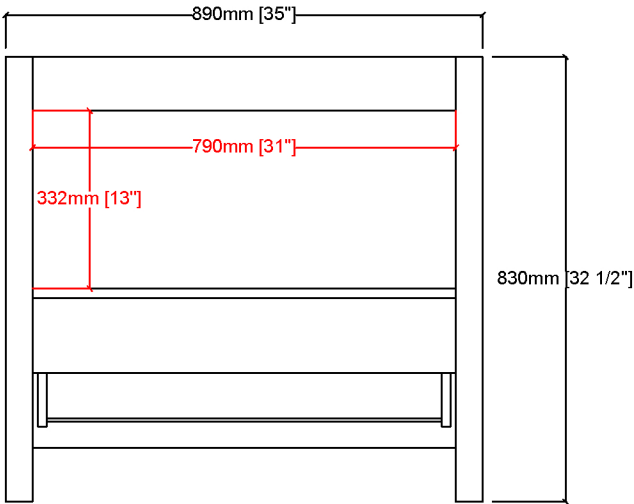
BACK VIEW
