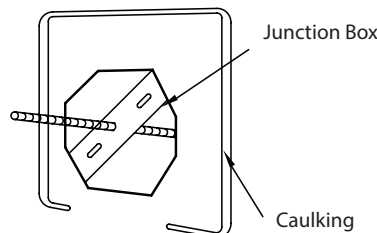
Fig.3 Sealing
