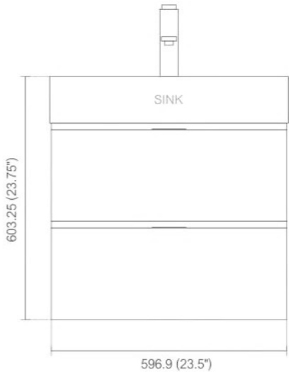
. FRONT ELEVATION
