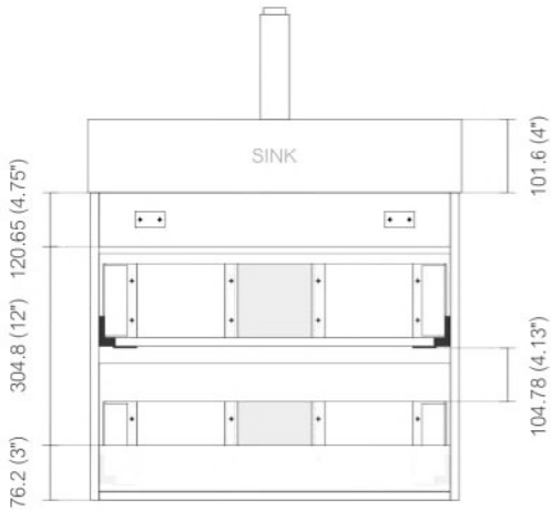
. BACK ELEVATION
