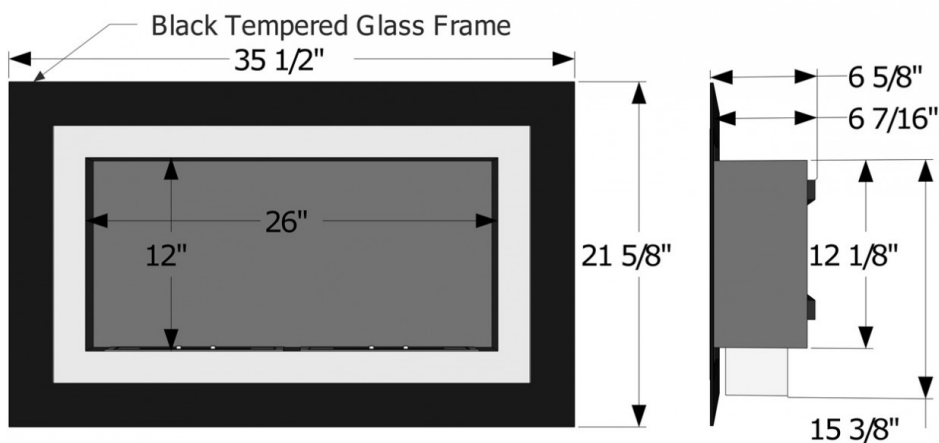
Villa Fireplace Dimensions
