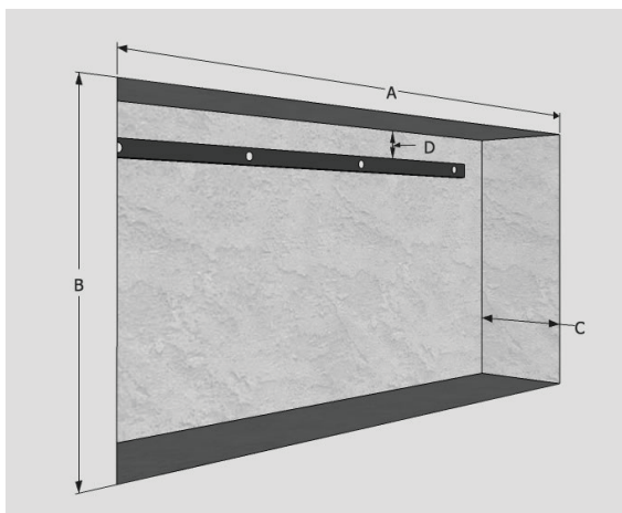
Recessed Opening Sized for Villa Fireplace
