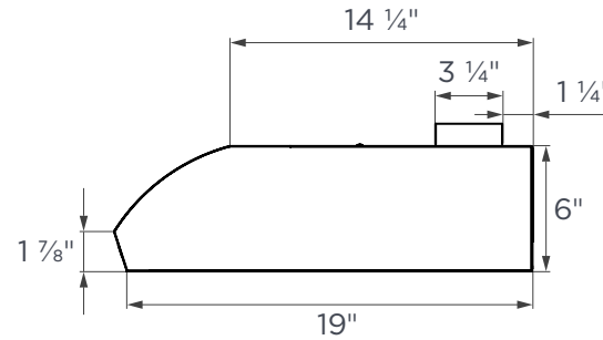
SIDE
