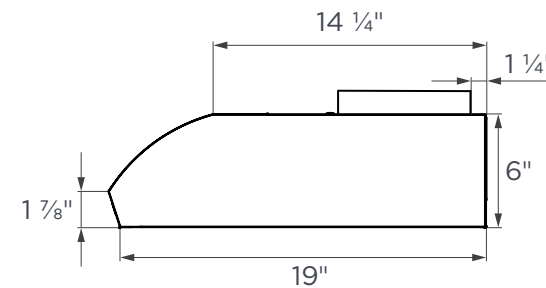
SIDE
