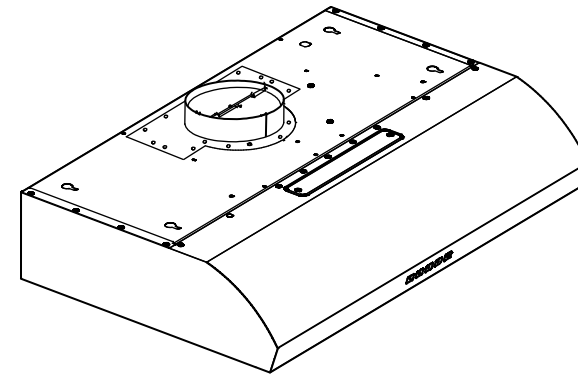
TOP ROUND EXHAUST ADAPTER
