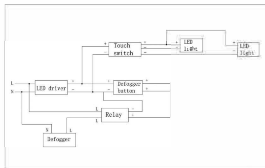
Circuit diagram
