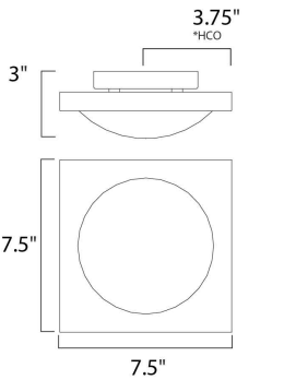
*height from center of the outlet to the top of the fixture
