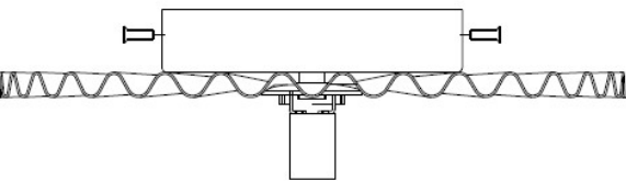
DRAWING 2- GLASS INSTALLATION
