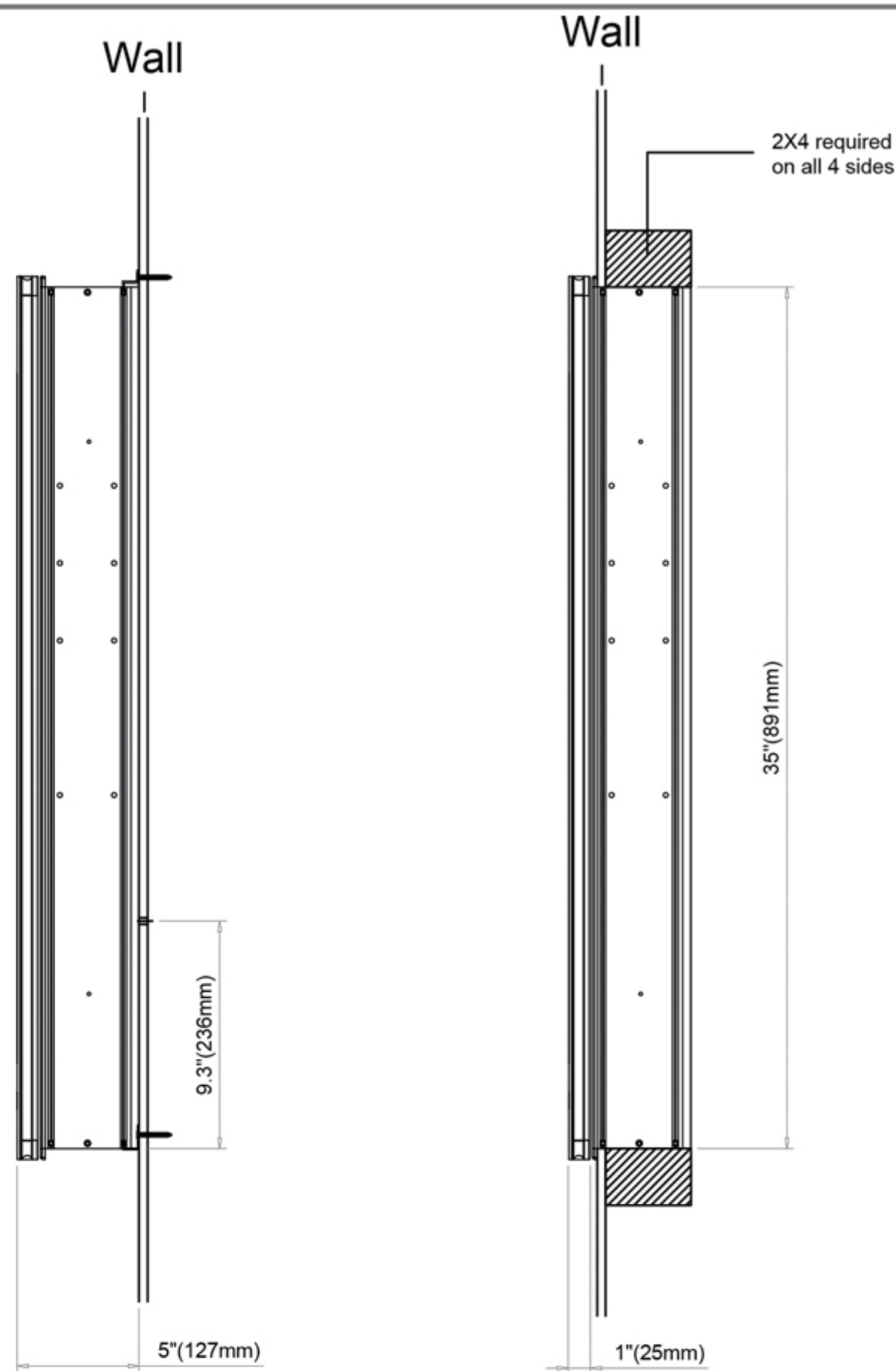
Surface Mount
