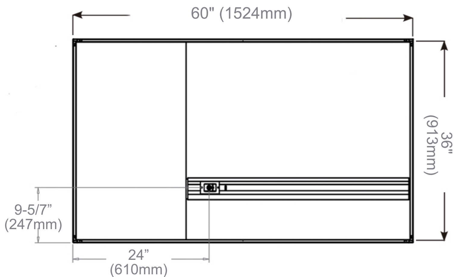
Back of Cabinet - Wire Access Location
