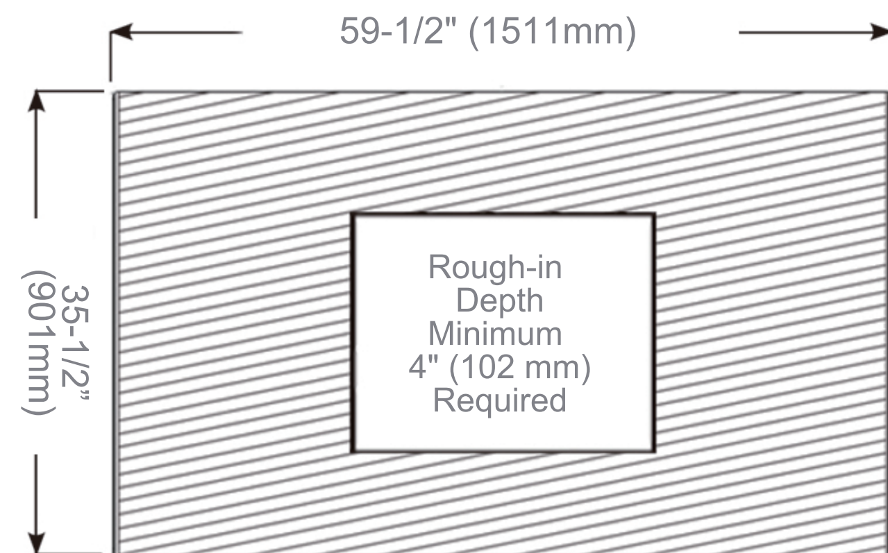
Rough-in Dimensions
