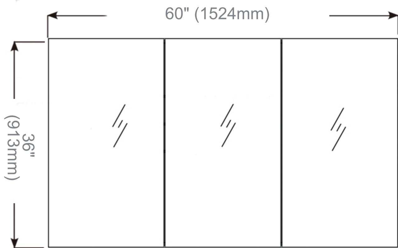
Cabinet Dimensions
